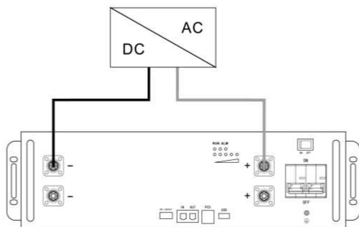
Figure 5-2: Single Battery Connection
